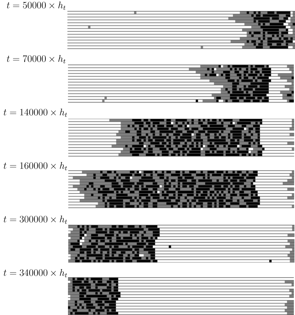
Figure 7. Time progress of a pulsing state for the thirteen-lane model of size N = 100 , \alpha_+ = 4.0 \text{ s}^{-1} and no flux on the plus end; otherwise the parameters are as in table 2 and the boundary conditions as in (5). The sequence of filling (top three frames) and emptying (bottom three frames) repeats approximately periodically. Observe that the pulse of high-density mixed particles propagates slowly to the left via diffusion of vacancies through the pulse. Grey indicates plus-type particles (that move to the right) while black indicates minus-type particles (that move to the left). The white regions indicate vacancies.
