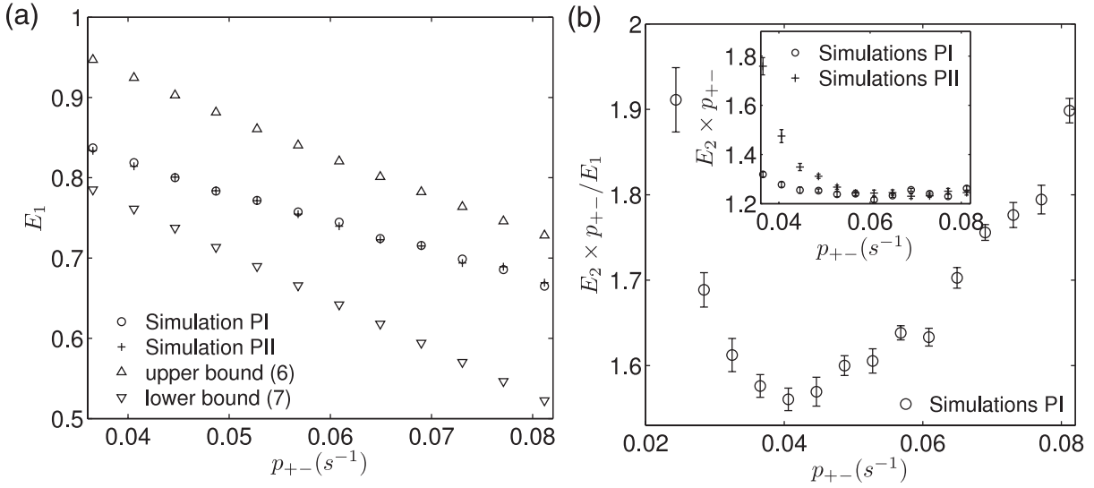
Figure 6. Illustration of E_1 and E_2 when varying p_{+-} . (a) shows that the arrival efficiencies E_1 in the two lane-change protocols, PI and PII, behave similarly, when varying p_{+-} with the approximate upper bound from (6) and lower bound from (7). (b) shows the balance between the delay ratio and the arrival efficiency quantified as E_2 \times p_{+-} / E_1 for protocol PI; the inset shows the comparison between two protocols PI and PII of the delay ratio E_2 \times p_{+-} ; error bars are indicated. Simulations were done by averaging over 10 runs using the Gillespie algorithm in a time interval [T_0, T] = [500 \text{ s}, 3000 \text{ s}] ; other rates are defaults, as in table 2, and we used the boundary conditions of (5).
