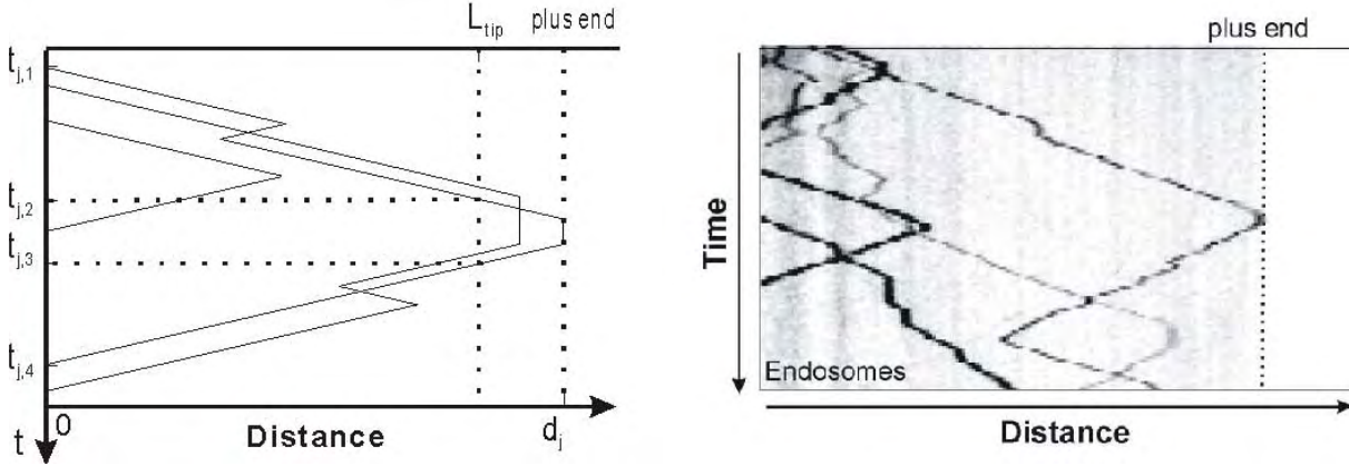
Figure 5. Typical motion of three particles injected into the system (left panel). We show the times t_{j,m} , m = 1, \dots, 4 , for the j th particle. Particles that exceed L_{\text{tip}} are said to have entered the tip region. The kymograph (right panel) shows the motility of early endosomes that were visualized by photo-activation of the endosome marker paGFP-Rab5a [21] in subapical regions of a cell of the fungus Ustilago maydis . Note the similarities in the two panels of the trajectories of motions.
