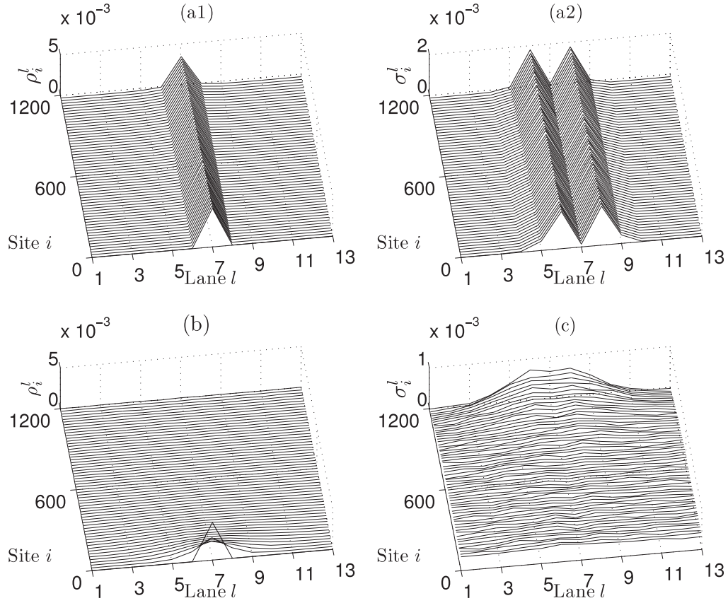
Figure 2. Densities of plus- or minus-type particles corresponding to the default parameters in table 2 and boundary conditions in (5) except that the lane-change rates when unblocked are varied and there is injection only in one lane (namely \alpha_+^7 = 1 \text{ s}^{-1} and \alpha_+^l = 0 for l \neq 7 ). (a1) and (a2) show the inhomogeneous densities of plus- and minus-type particles respectively, when p_{\pm,u} = 0 , i.e., particles only change lanes after collisions; (b) (resp. (c)) shows cross-lane diffusion leading to a more homogeneous density of plus-type (resp. minus-type) particles away from the boundaries with lane-change rates when unblocked as p_{-,u} = 0 , p_{+,u} = 4.335 \text{ s}^{-1} (resp. p_{-,u} = 0.4335 \text{ s}^{-1} , p_{+,u} = 0 ). In all cases the densities near the tip (not shown) are high.
