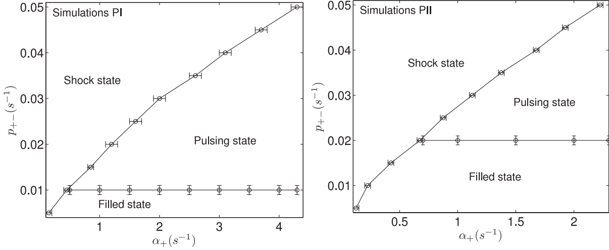
Figure 10. Numerically obtained phase diagrams for lane-change protocol PI (left panel) and lane-change protocol PII (right panel). The other default parameters are as in table 2 and the boundary conditions are as in (5). Bars indicate the uncertainty of the borders between different states.
