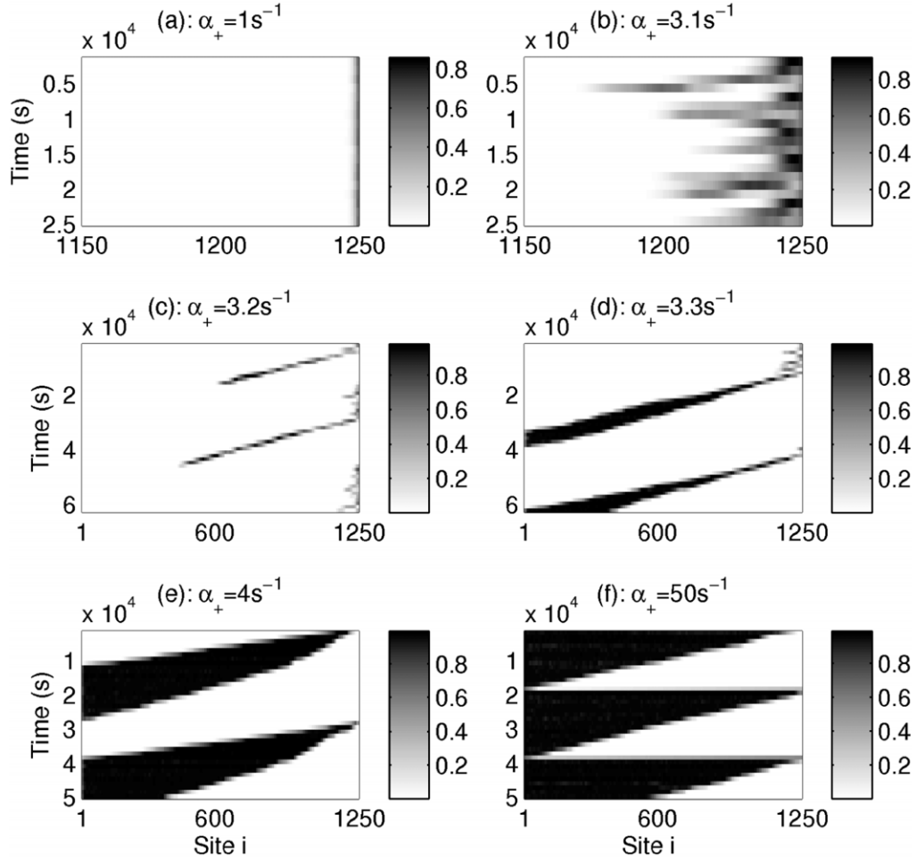
Figure 9. Each horizontal line represents a time average of the occupancy \sum_{l=1}^M (\tau_{-,i}^l + \tau_{+,i}^l) / M over blocks of length 1260 s in the homogeneous thirteen-lane model ( M = 13 ) with the injection rate \alpha_+ indicated (other rates are defaults). In (a), the model with a small total injection rate reaches its stationary state with a small number of particles accumulated in the tip. (b)–(d) show the density–time courses for injection rates near the critical value. In (d)–(f), pulsing states appear where the accumulation moves away from the plus end and simultaneously grows.
